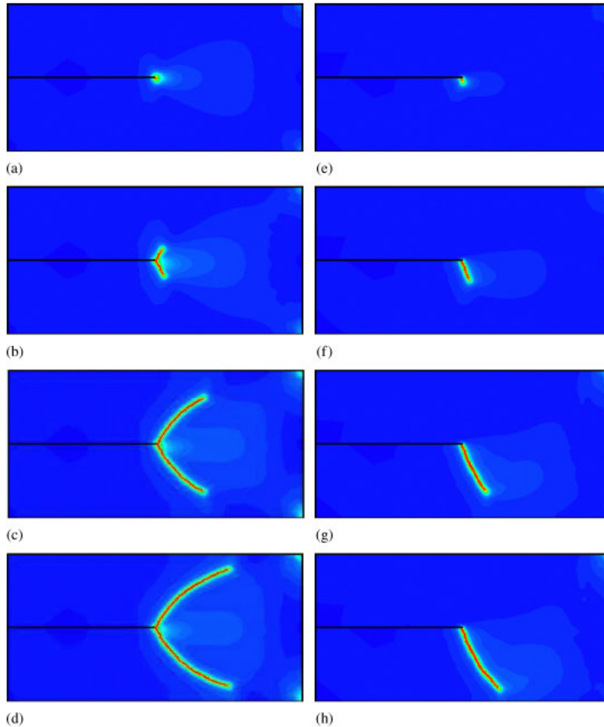
Figure 16. Pure shear test. Crack patterns of the three-field formulation with model II version (62) are depicted on the left-hand side at the deformation state: (a) u=9.0 \times 10^{-3} mm; (b) u=11.0 \times 10^{-3} mm; (c) u=15.0 \times 10^{-3} mm; (d) u=17.0 \times 10^{-3} mm. Results obtained with model II version (63) are given on the right-hand side at the deformation state: (e) u=9.0 \times 10^{-3} mm; (f) u=11.0 \times 10^{-3} mm; (g) u=15.0 \times 10^{-3} mm; and (h) u=17.0 \times 10^{-3} mm.
