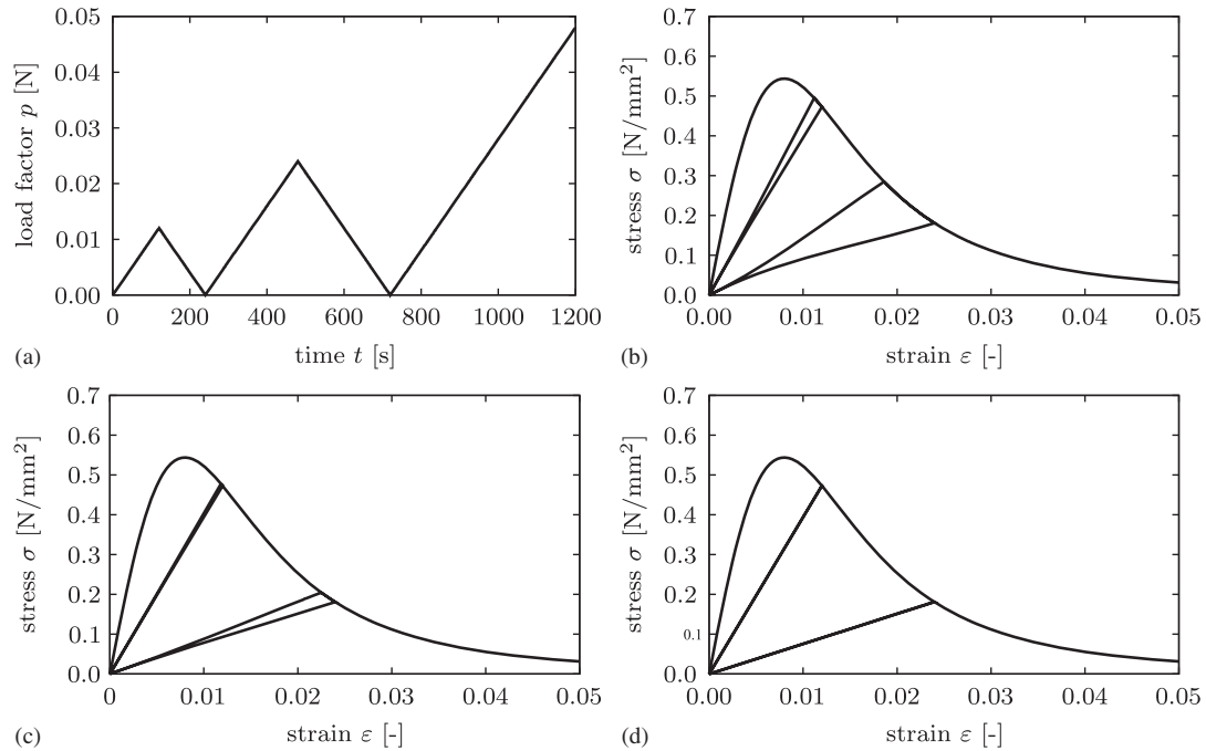
Figure 8. Model I: Rate-independent setting with approximated indicator function. (a) Cyclic loading and stress–strain curves for (b) \epsilon=0.01 ; (c) \epsilon=0.05 ; and (d) \epsilon=2.0 . For small penalty parameters \epsilon , the model shows a non-physical hysteresis in unloading–reloading.
